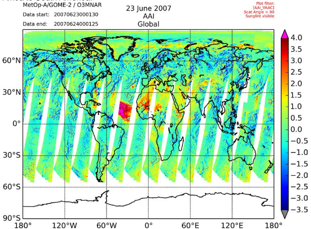
Figure 4: Absorbing Aerosol Index (AAI) from GOME-2 for June 23 rd 2007.
