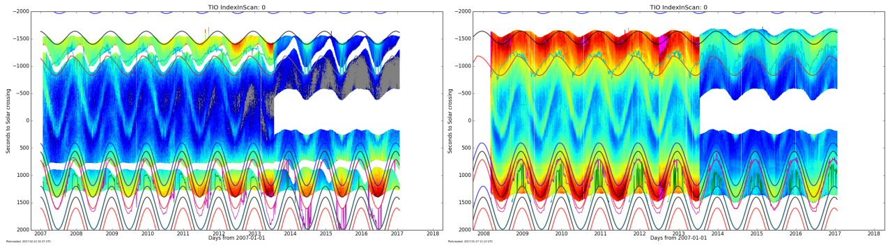
Figure 5.6: Hovmöller-diagram (TIO against time) showing the AAI for every Eastern pixel throughout the GOME2-A operational period (MSC left, PMD right). The data is deseasonalised. Sinusoidal curves indicate the top, centre and bottom location of the three Gaussian functions. The white gaps structures on the top and bottom are caused by the C-shape filter. From July 2013 onward the sun glint moves to the Eastern most pixel due to the GOME-2 small swath mode and is also filtered out.
